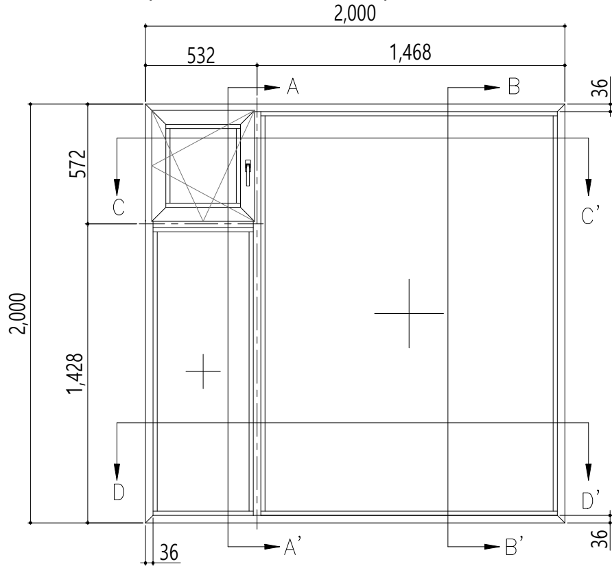
ELEVATION (INTERIOR VIEW)
