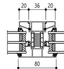
section D-D'
